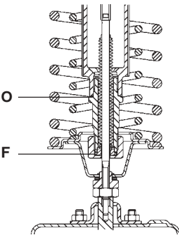
Fig. 12c - DN32 ÷ 50 (1 1/4" ÷ 2")
