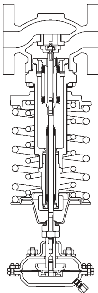
DN32 ÷ 50 ( 1\frac{1}{4} " ÷ 2")
