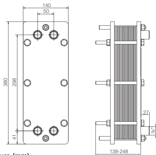
Misure (mm)
